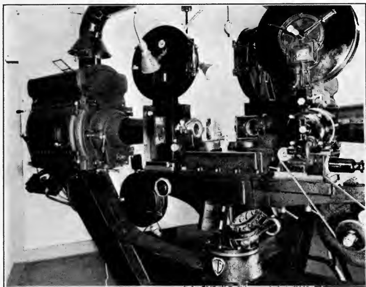
FIG. 3. Quarter front view, showing means of rotating the projector and optical bedplate about the optical axes of side projectors.
